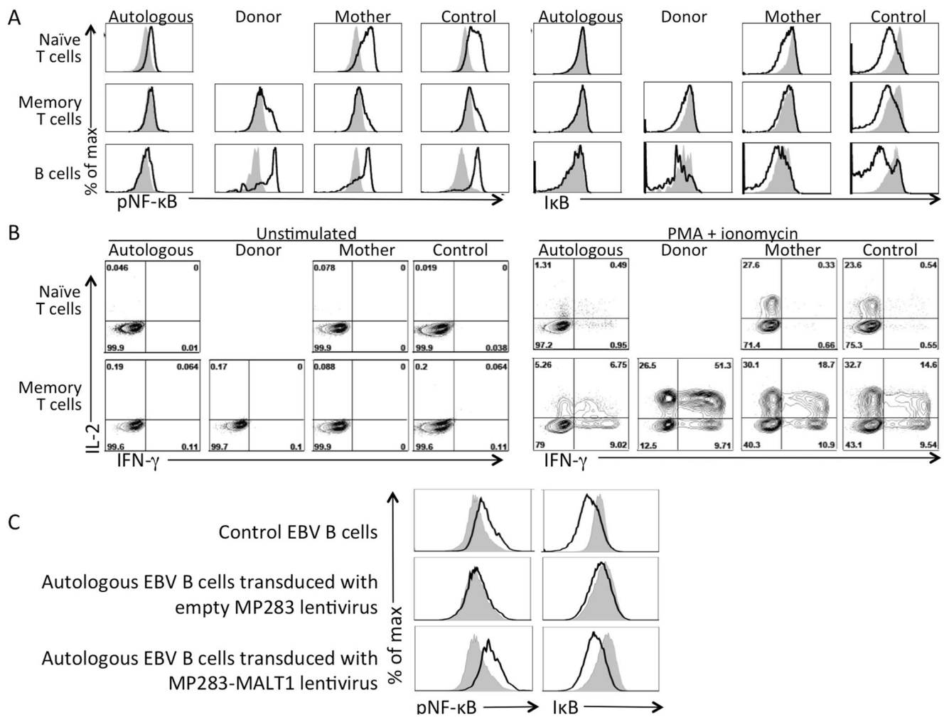
Fig. 3 a , Intracellular phospho-NF- \kappa B and I \kappa B in gated unstimulated ( gray shading ) vs. PMA and ionomycin stimulated ( black line ) naïve and memory CD3 + T cells and CD19 + B cells from the patient, including patient autologous (TRA2G9 + ) and donor-derived (TRA2G9 - ) cells; also analyzed were cells from the mother and a healthy control. b , T cell expression of intracellular IL-2 (y-axis) and IFN- \gamma (x-axis) without ( left panels ) and with ( right panels ) PMA plus ionomycin stimulation. c ,
