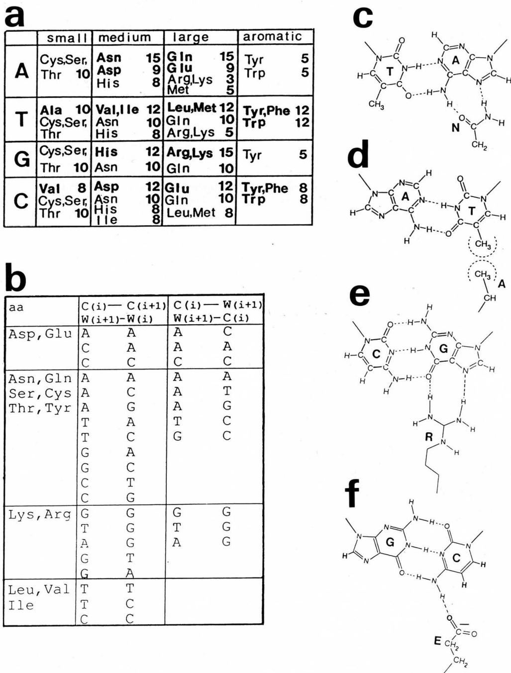
Fig. 1. Chemical code tables ( a and b ) and examples of amino acid–DNA base contacts ( c–f ). ( a ) The table for single amino acid–single base contacts. The ‘specific’ residue partners (see text) are shown in bold, while non-specific partners are in plain text. Chemical merit points, semi-arbitrary numbers associated with particular contacts, are used to quantify the energy and specificity of a pairing between an amino acid residue and a nucleotide base. For example, the interaction of Arg (to G), which is particularly favorable and specific, with the residue receives 15 merit points, while the interaction between Ser (to any base), which is less specific, is given 10 points. These are combined with stereochemical merit points (Figure 2) to compute a DNA–protein interaction score, as described in the text. ( b ) Table for the bridging of two bases by single residues: two bases on the same DNA strand (left) and two on different strands (right). ( c–f ) Base–residue contacts Asn–A, Ala–T, Arg–G and Glu–C are shown. All of these use hydrogen bonds except Ala–T, which involves a hydrophobic interaction.
